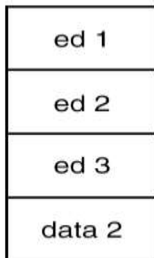
process P_2
